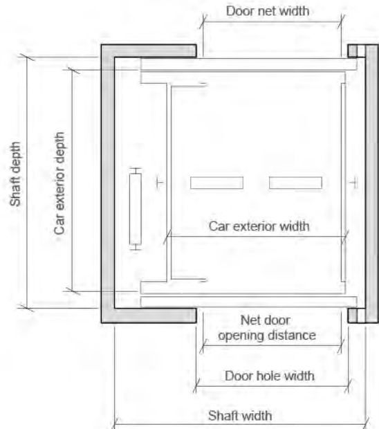
Shaft layout drawing
